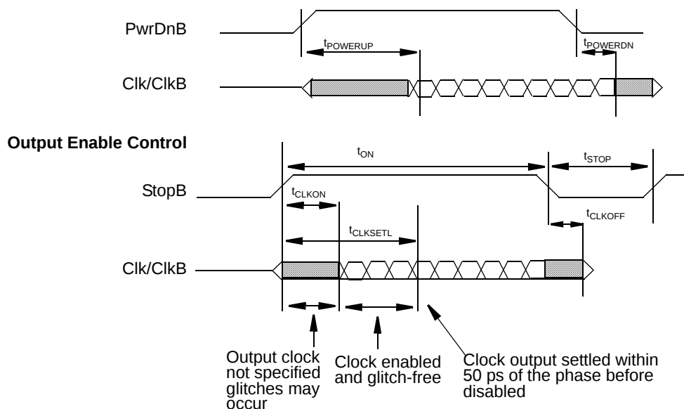
Figure 5. State Transition Timing Diagrams
